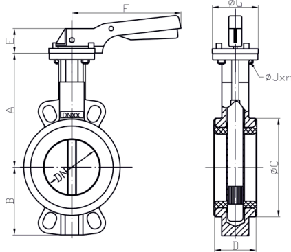
Lock lever 497 DN32 - DN150
