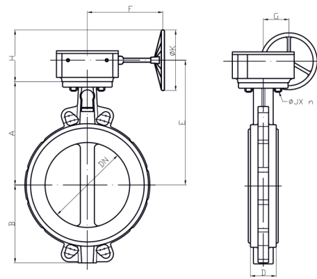
Gearbox 497 DN350 - DN600
