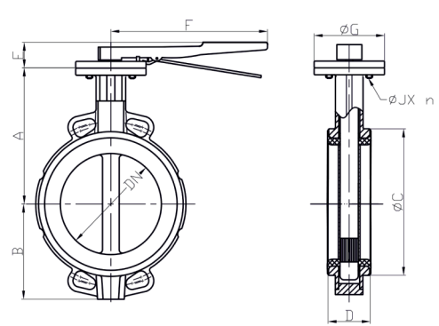
Lock lever 497 DN200 - DN300
